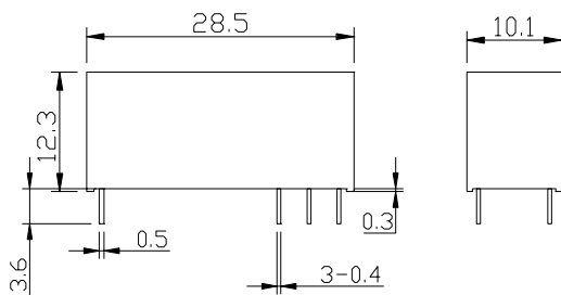
SPDT – 1 form C
